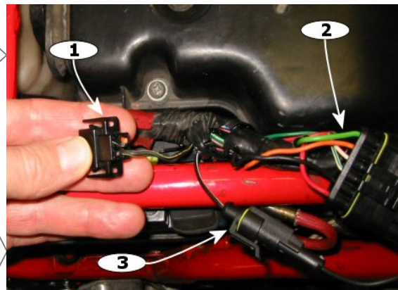
1: Powervlve Control Unit / 2: CDI-unit / 3: HT-coil
